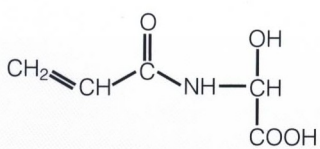
Acrylamido glycolic acid 16
