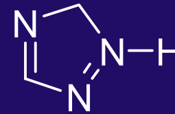
1.2.4-Triazole
