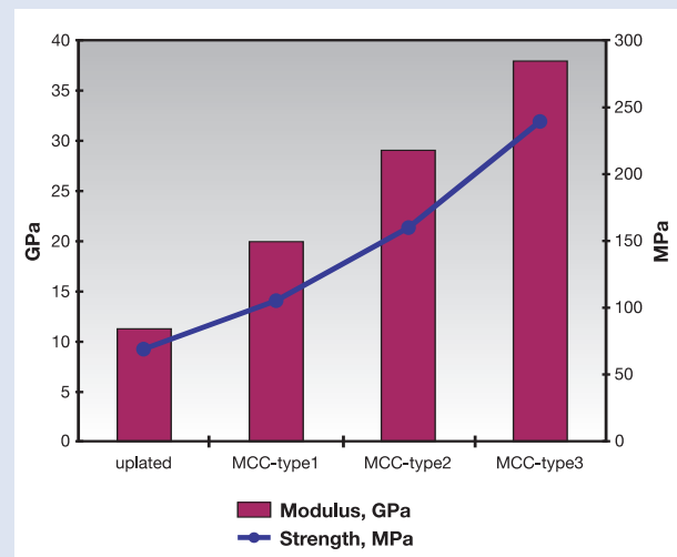
Graph 1. Shows tensile strength and tensile modulus values versus unplated NanoTool and three MC 2 construction types.
